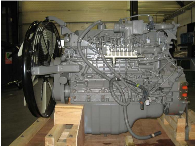
Isuzu 6HK1XY common-rail engine, 220 kW
